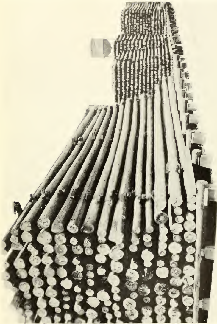
Well-graded poles in an air-seasoning yard. Each pile is high above the ground on treated piers and stringers. Heavy stickers, also treated with preservative, separate successive layers. The sanitation is excellent.
